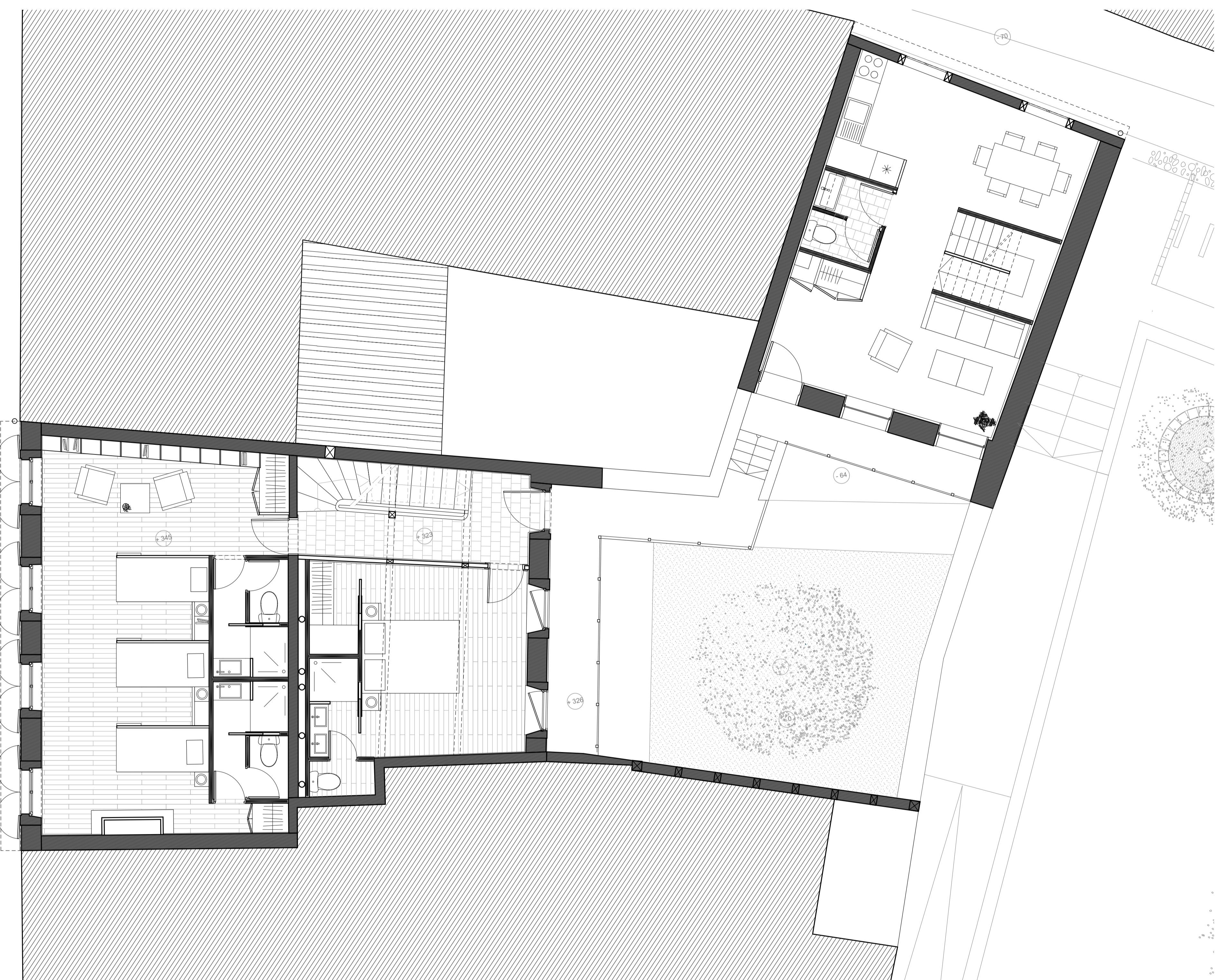
PLAN R+1 1:50
