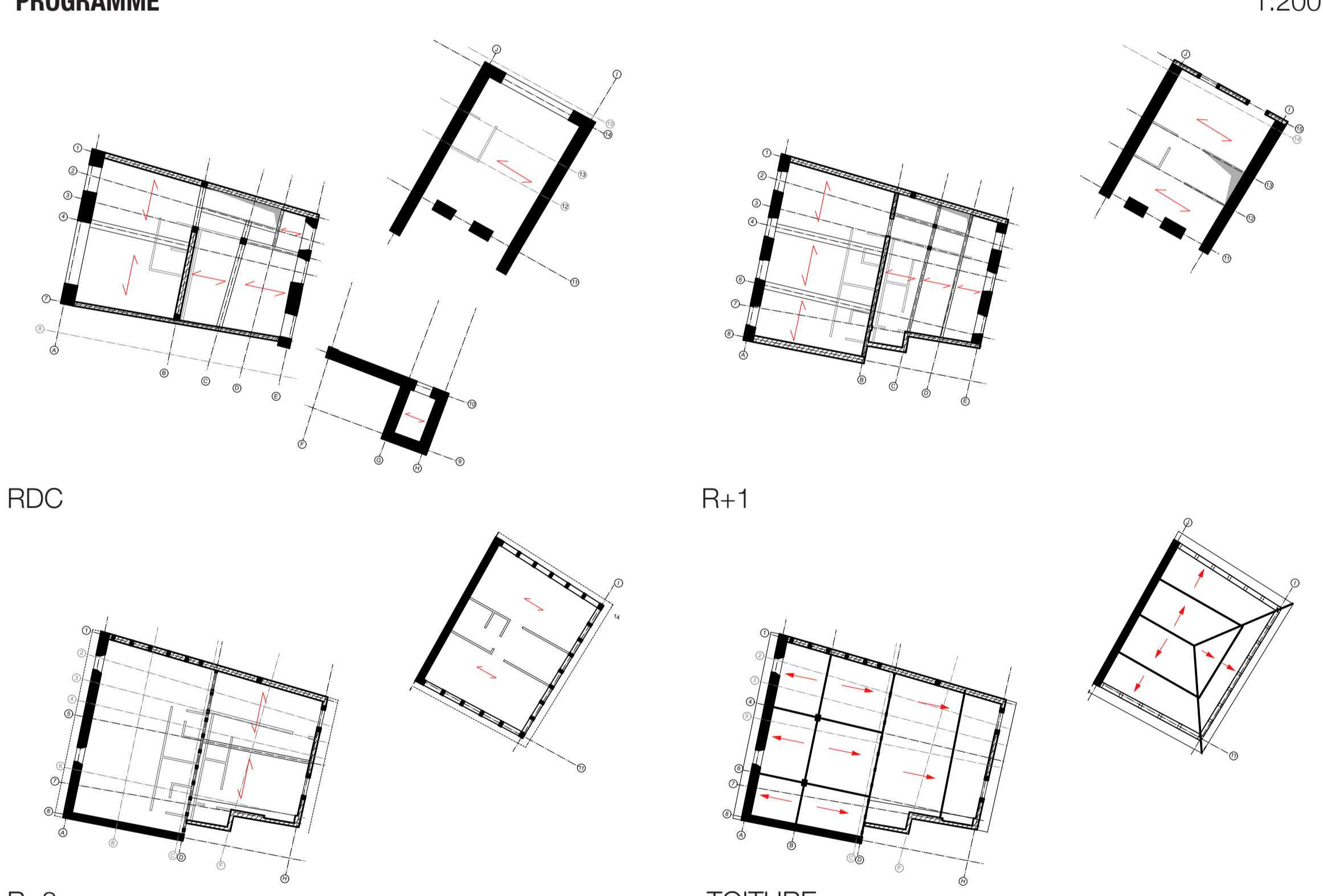
PLAN STRUCTURE 1:200
